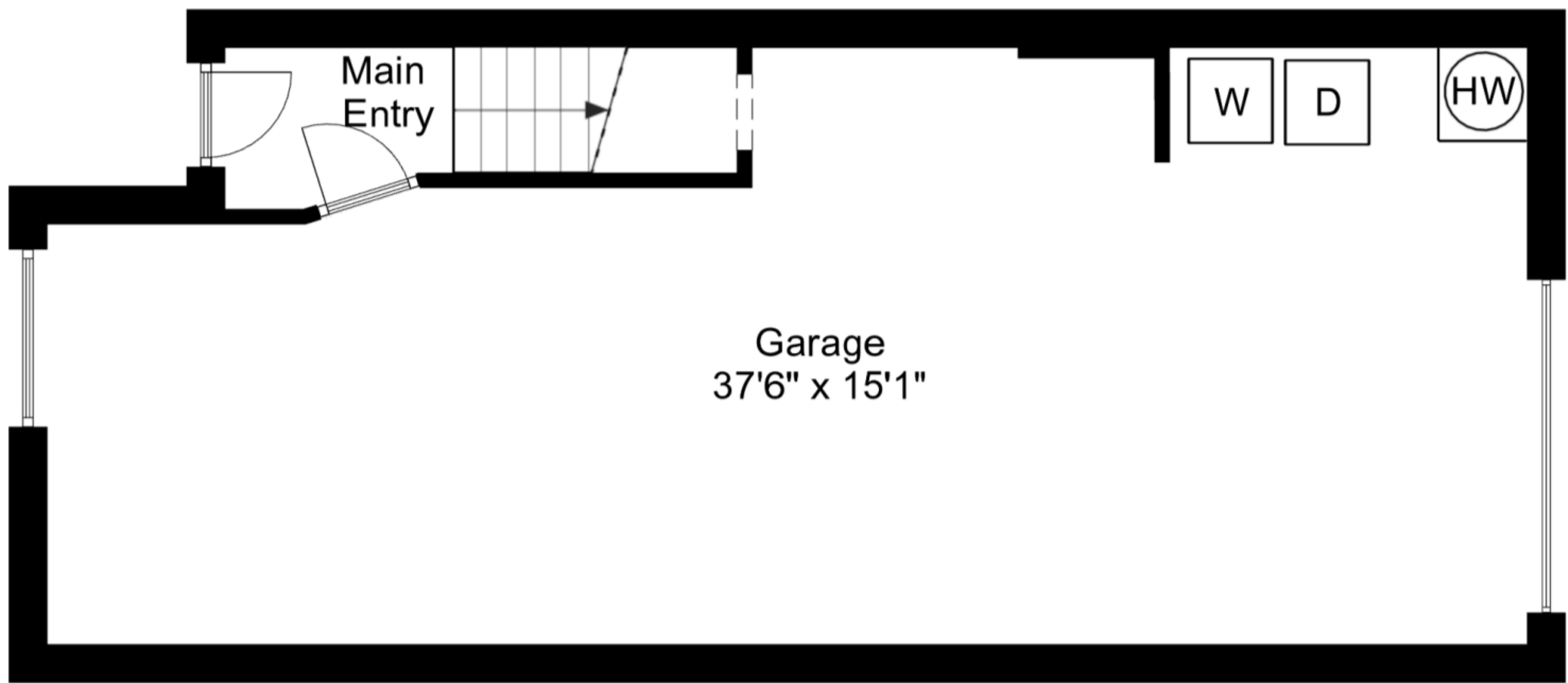
Lower Level
